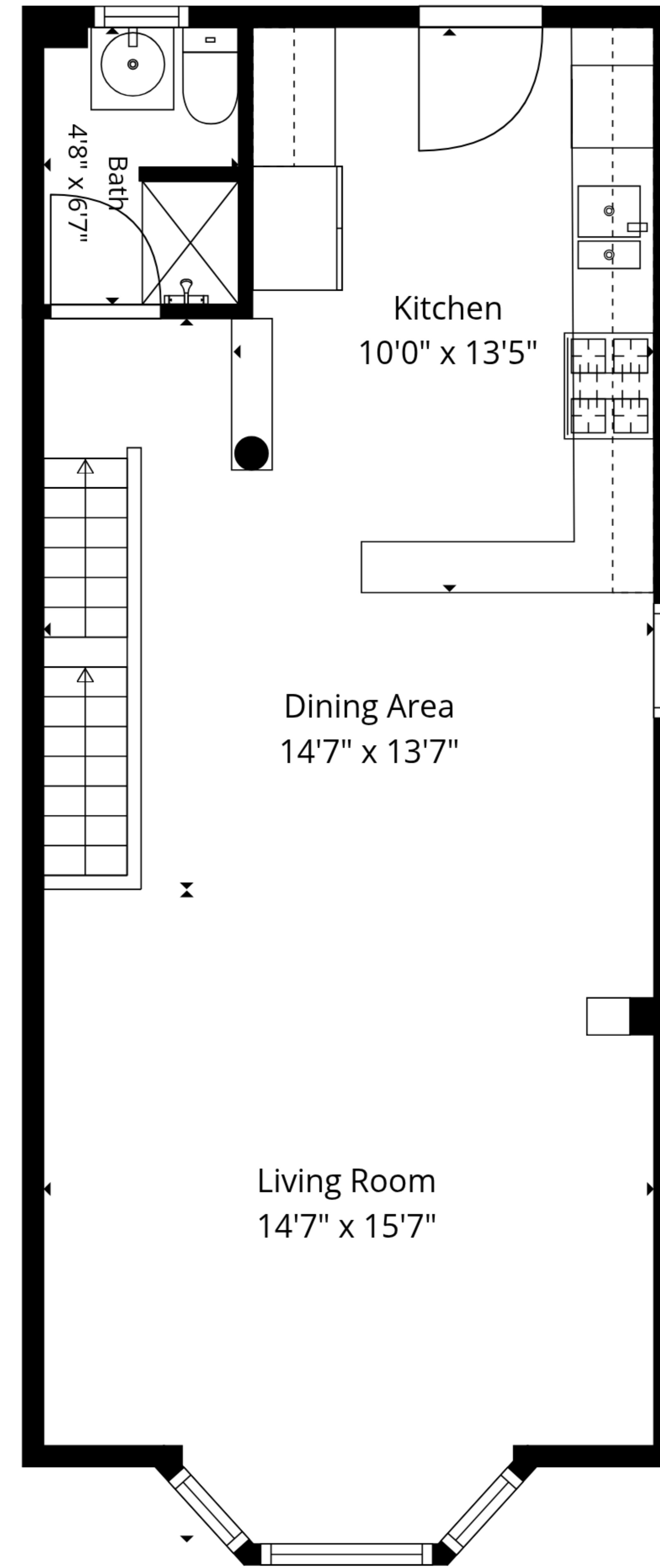
2nd Floor
