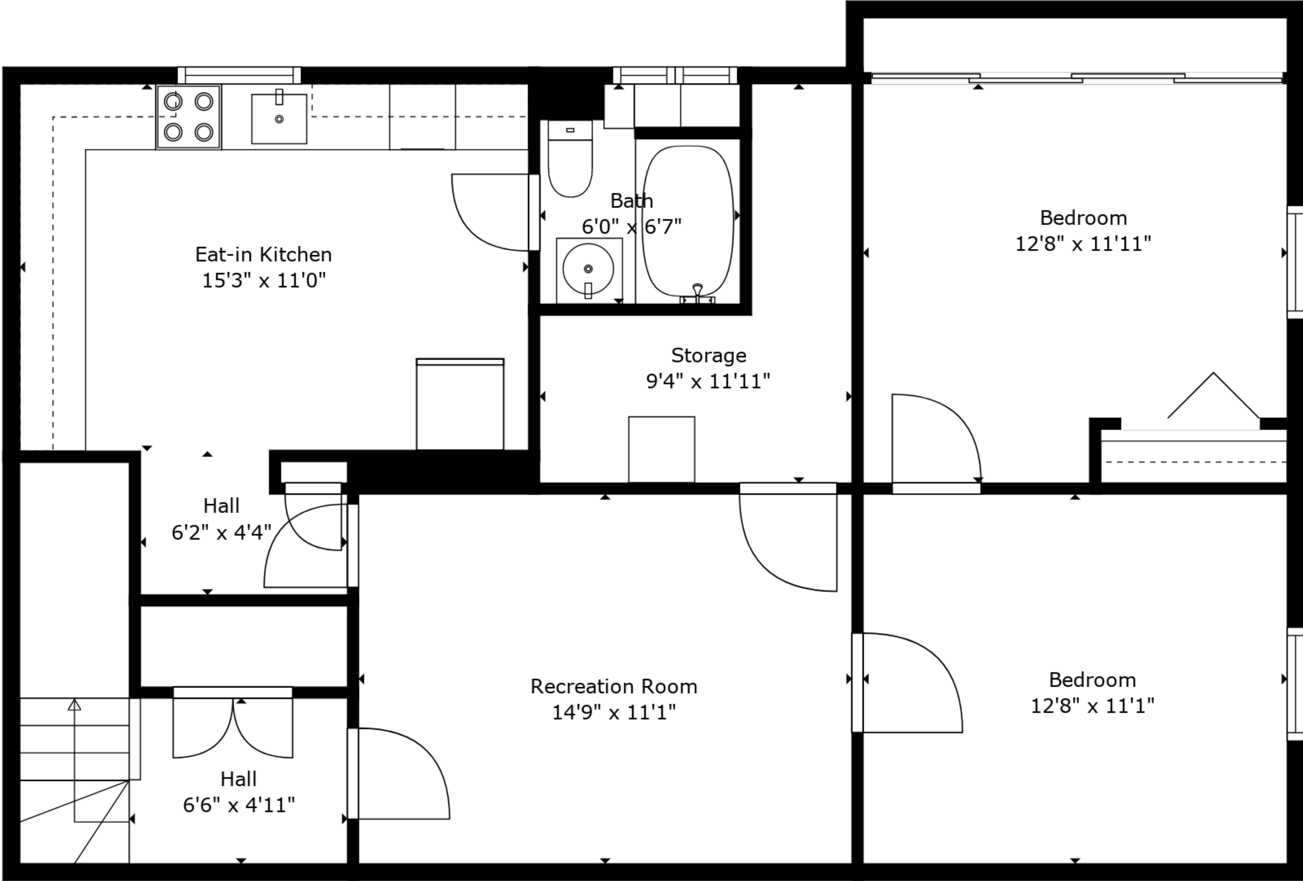
Lower Level
