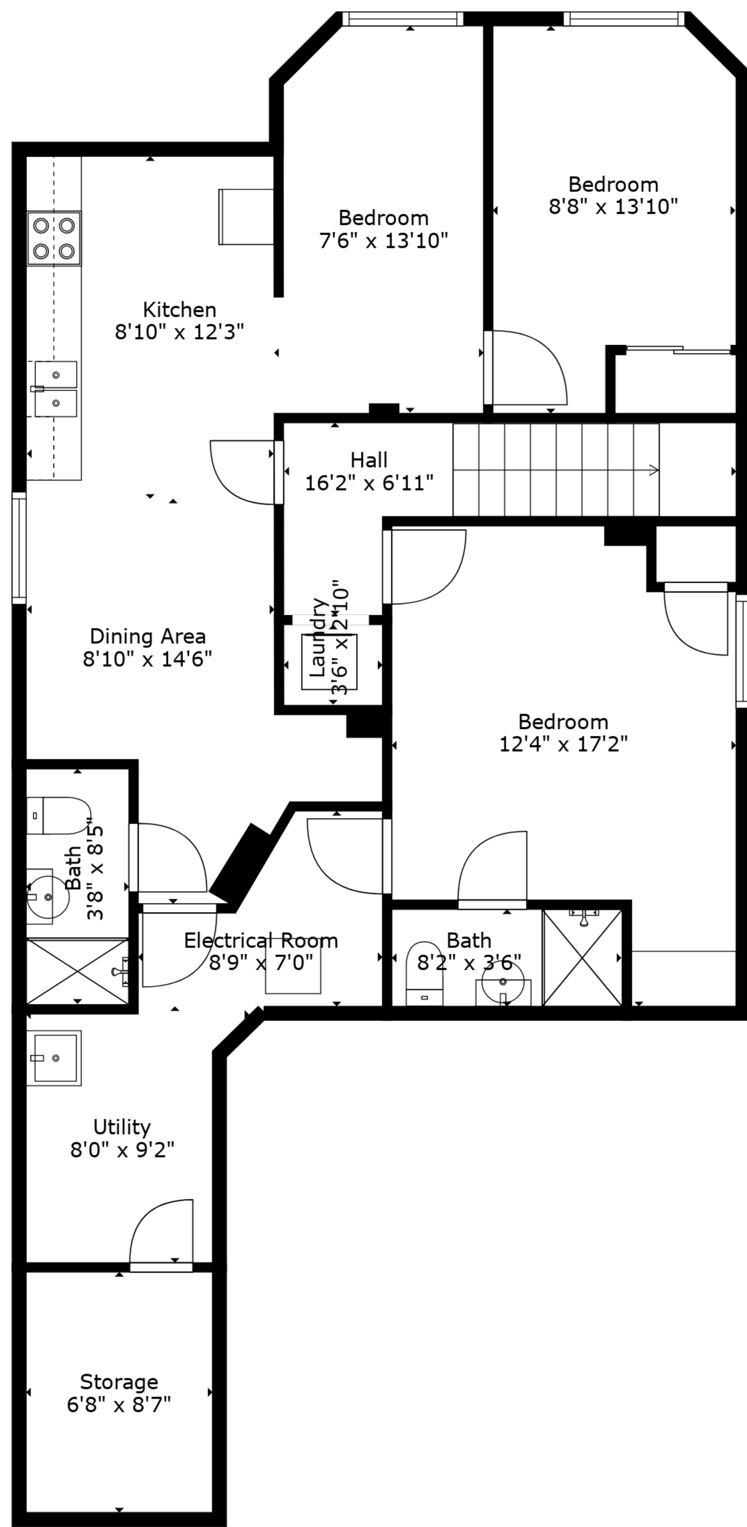
Lower Level
